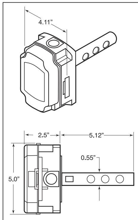
Figure 2 - Duct Sensor Dimensions
