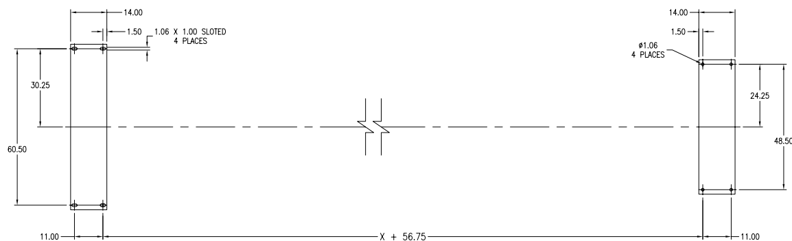
FOOTPRINT
