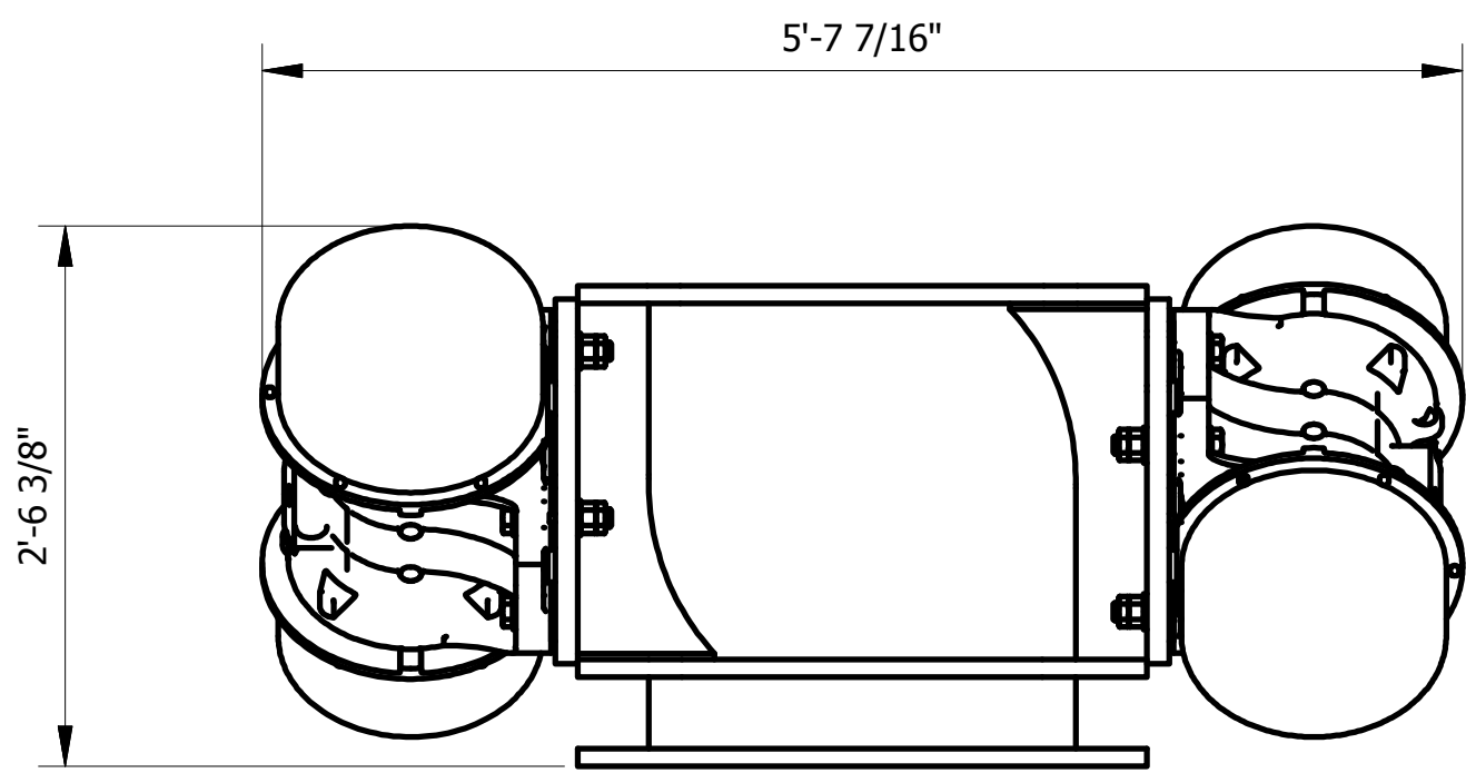
DRIVE ASSY (ITEM A117) SCALE 1 : 12
