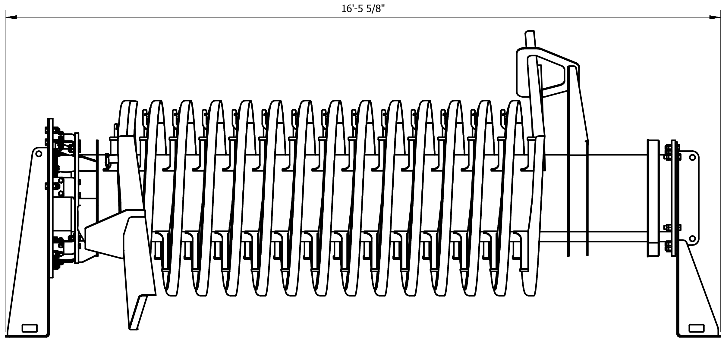
TOWER SHIPPING ARRANGEMENT (ITEM A115) SCALE 1 : 16
