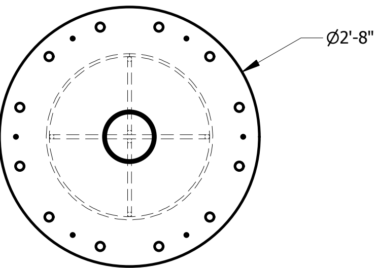
TOP ISOLATION PLATE ASSY (ITEM A116) SCALE 1 : 12
