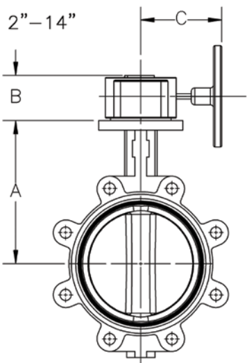
GEAR OPERATOR
